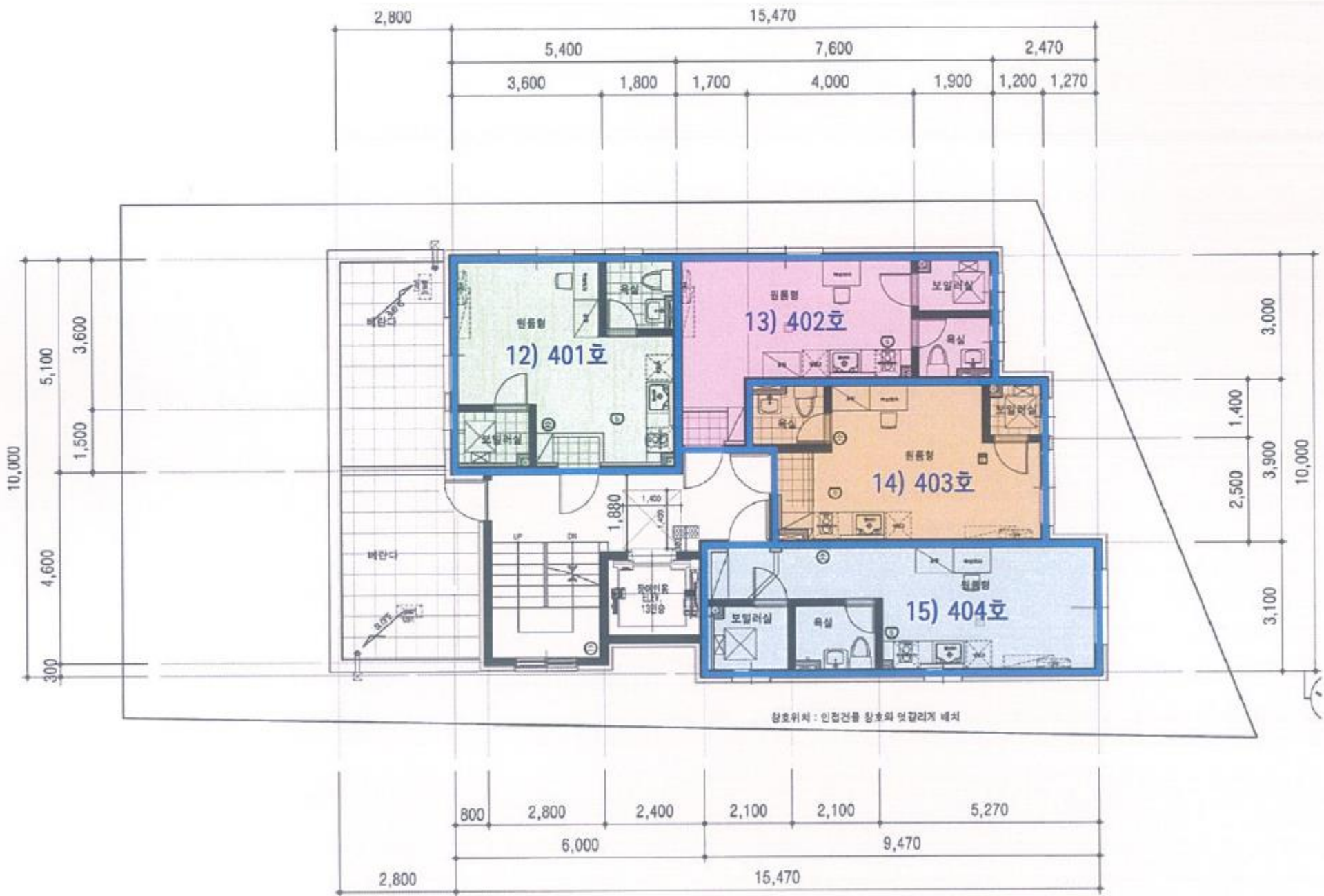
( 4층 )
