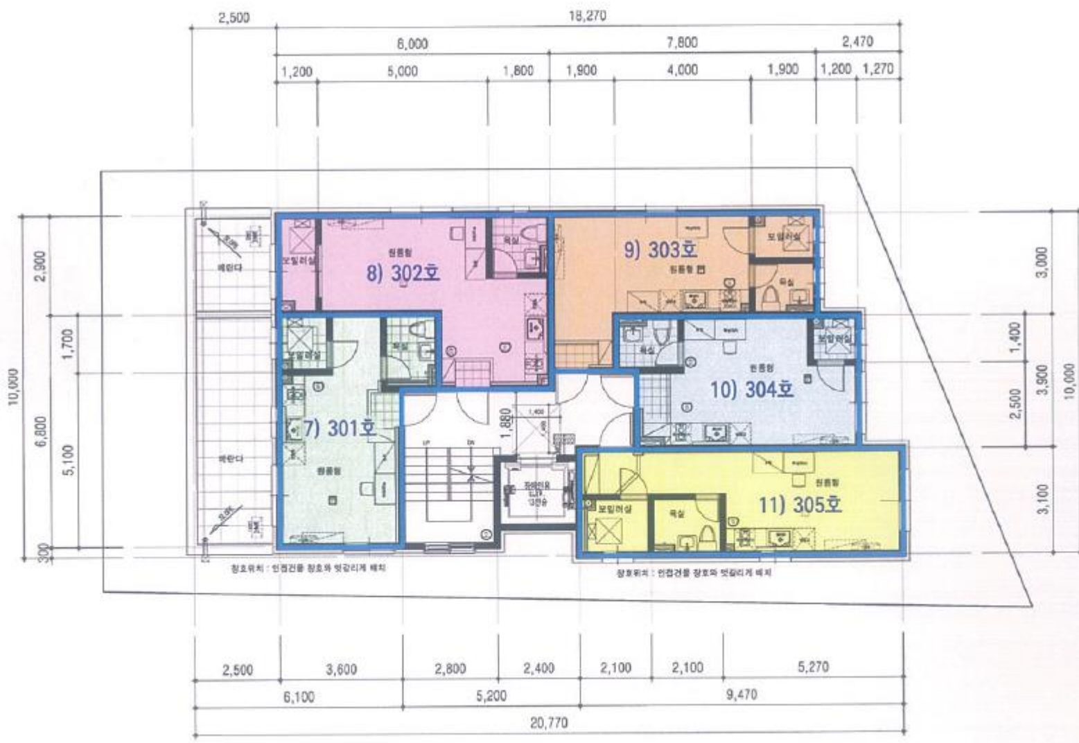
( 3층 )
